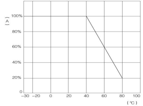
Load Current Derating v. Ambient Temperature
