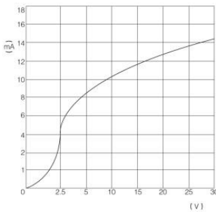
Input Current v. Control Voltage: 4 ~ 32VDC
