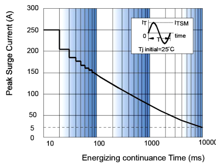
Max. Permissible Non-repetitive Peak Surge Current vs. Continuance time (SCR AC switch output)
