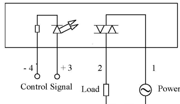
Wire Diagrams (Bottom View)
