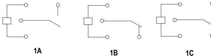
Wire Diagrams
