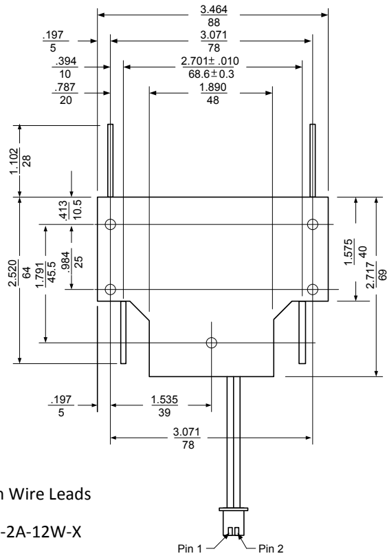
Dual Coil with Wire Leads Ex: PC25L-200-2A-12WD-X
