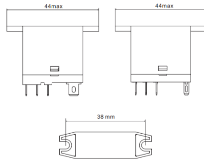
Top Flange Dimension
